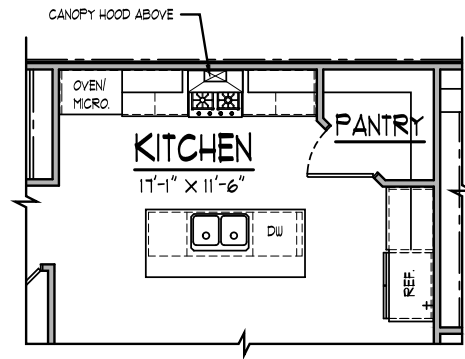
OPT. GOURMET KITCHEN NOT TO SCALE
