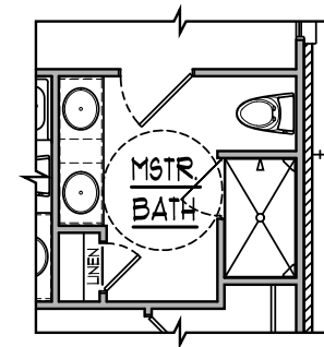
OPT. ROLL-IN SHOWER AT MASTER BATH NOT TO SCALE
