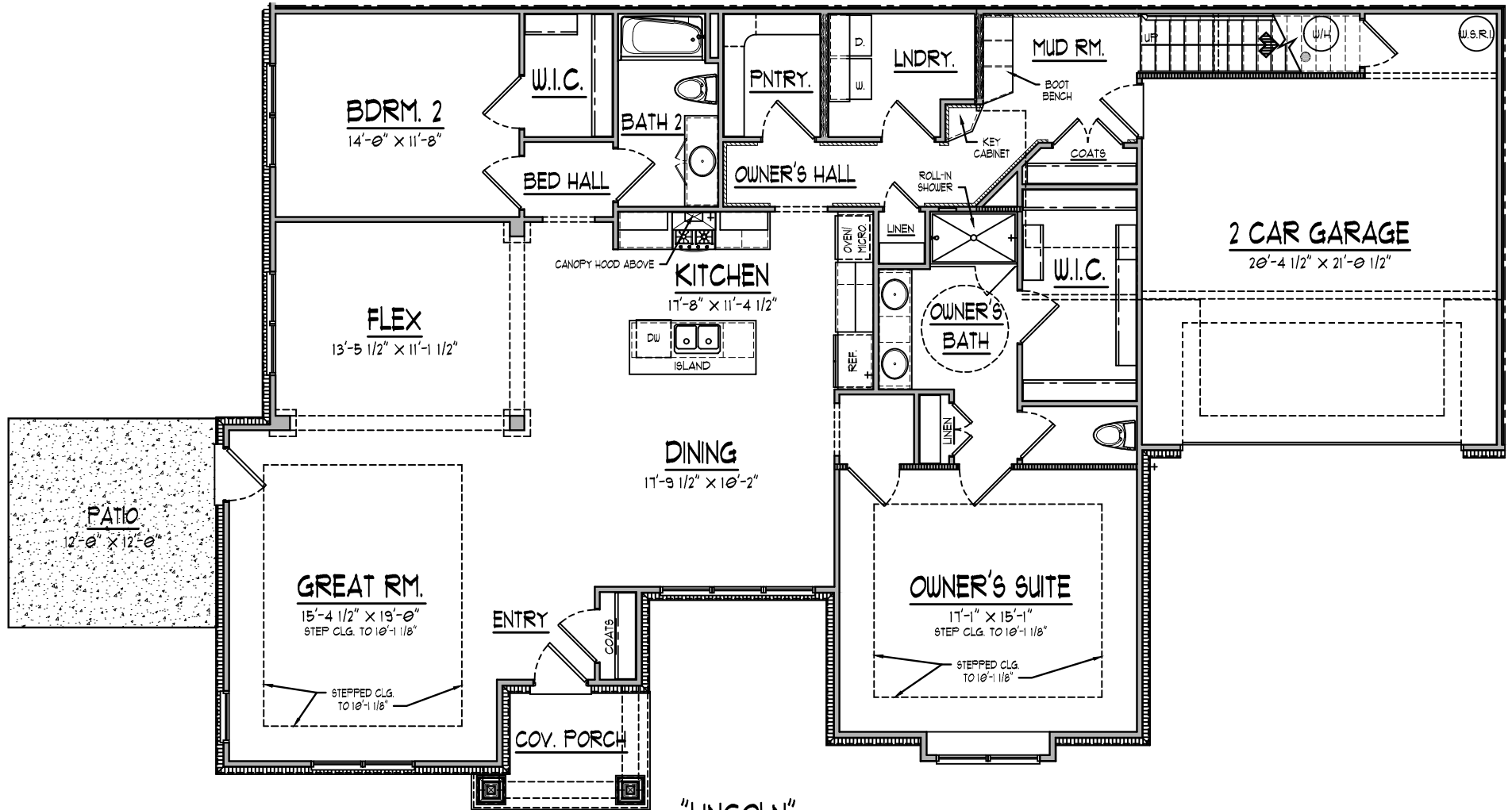
"LINCOLN" FIRST FLOOR PLAN SPEC AVAILABLE AT PRESERVE AT BROOKSIDE LOT #16 NOT TO SCALE 2,119 SQ. FT. (FINISHED)
