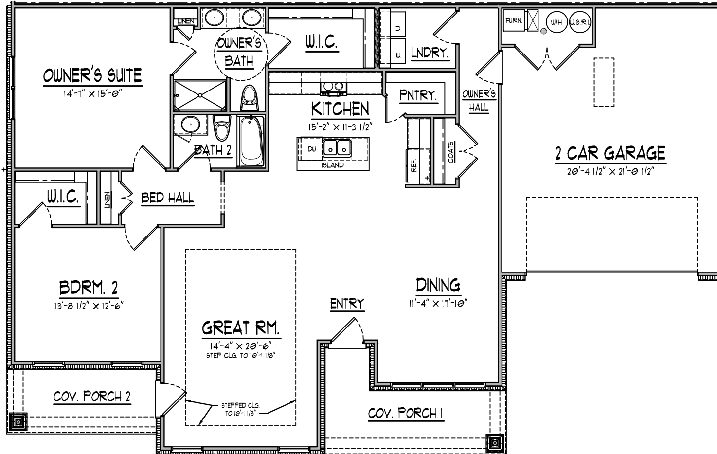
"MONTGOMERY" FIRST FLOOR PLAN SPEC AVAILABLE AT PRESERVE AT BROOKSIDE LOT #13 NOT TO SCALE 1,691 SQ. FT. (FINISHED)
