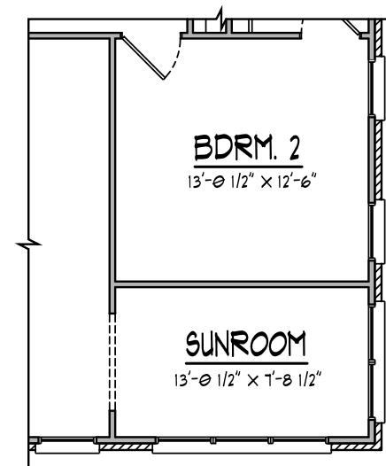
OPT. SUNROOM ILO COV. PORCH 2 FIRST FLOOR
