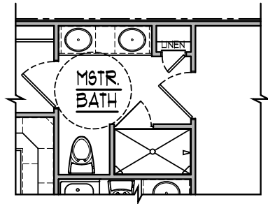
OPTIONAL ROLL-IN SHOWER AT MASTER BATH
