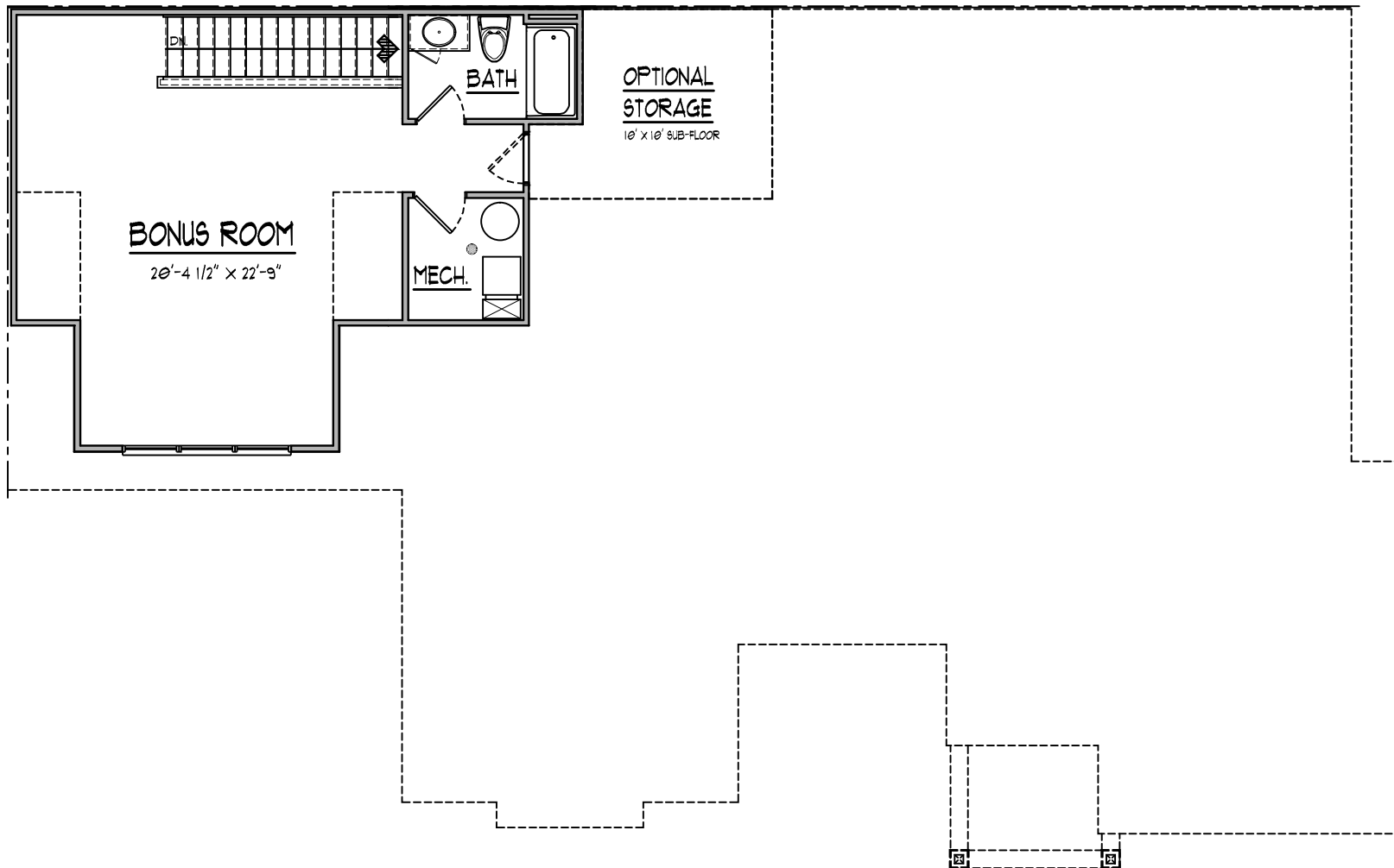
LINCOLN BROCHURE PLAN OPTIONAL BONUS ROOM AND OPTIONAL FULL BATH NOT TO SCALE 521 SQ. FT. (FINISHED)
