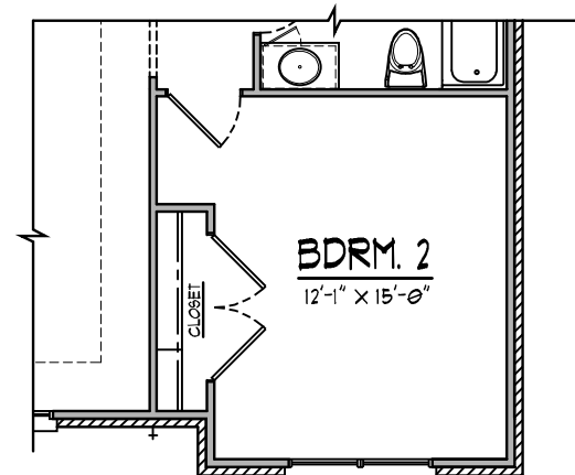
OPTIONAL BEDROOM 2 EXTENSION FIRST FLOOR
